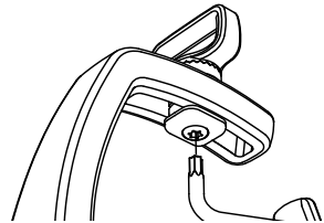
Screw for lateral adjustment and stirrup attachment
